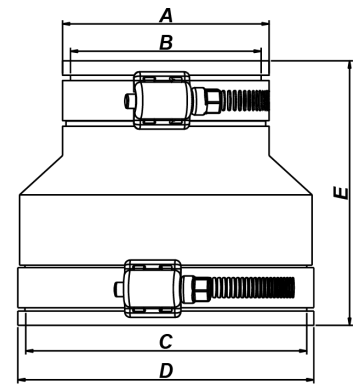
Reducing Flexible Couplings
