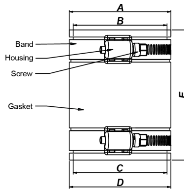
Flexible Couplings
